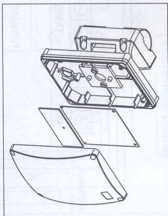
Fig. 8. MCB-200 - Transmitter unit with binding band.
