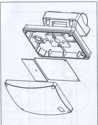
Fig. 7. MCB-200 - Receiver unit with binding
