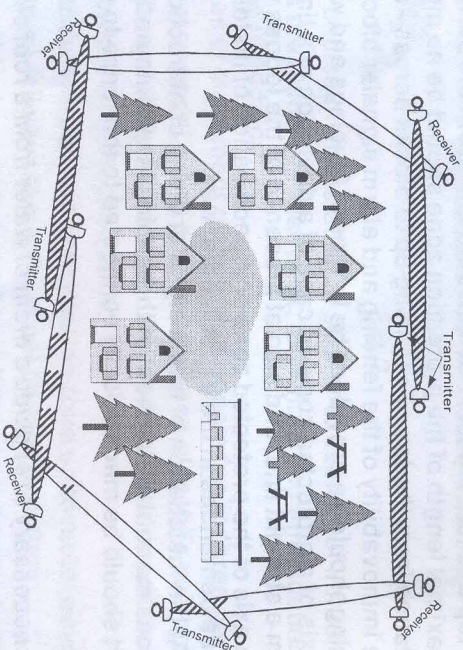
Fig. 4. Overlapping Angle and Range Installation of MCB-200 systems for area protection.
